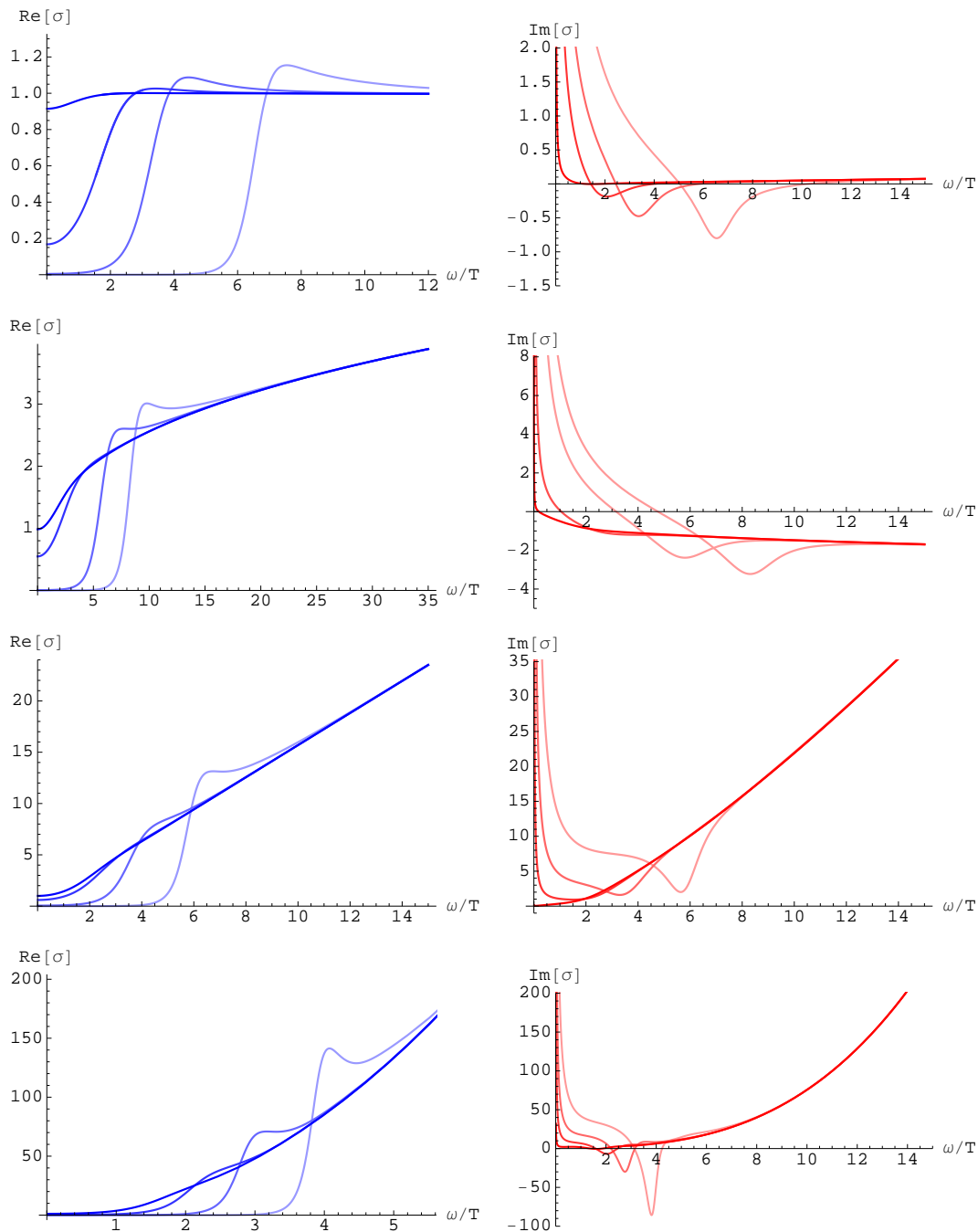
Figure 7. Real and imaginary parts of the conductivity for the four systems (from top to bottom: \text{AdS}_4 , D2/D6, D3/D7 and D4/D8), plotted for various values of the dimensionless chemical potential \mu/T (corresponding to the dots in figure 2).
